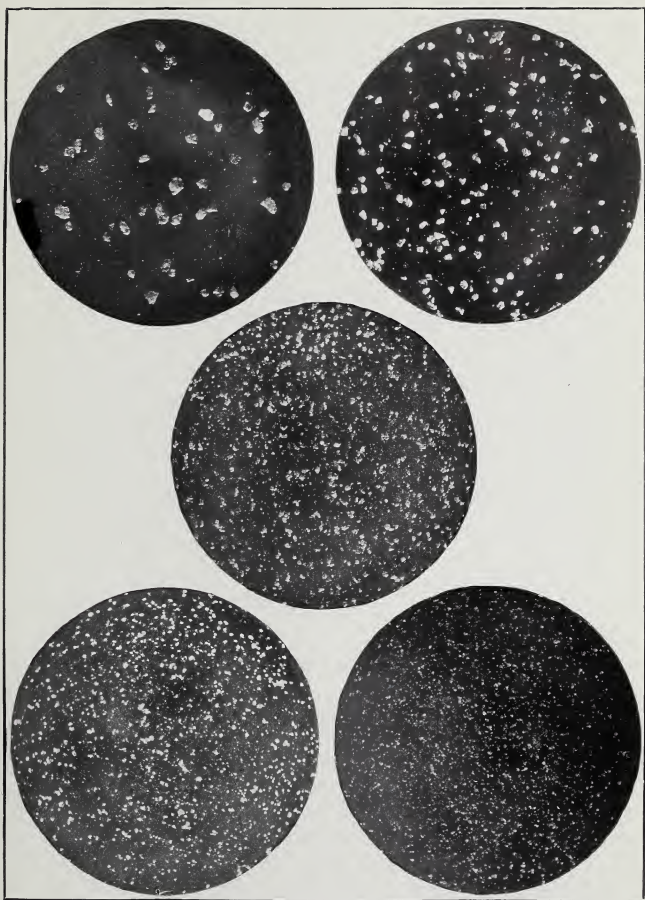
FIG. 47.—Cement, \times 40 .
